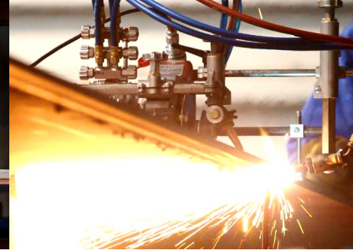
Chamfering (1:4 ratio bevelling) using single torch
