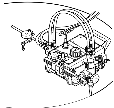
Y-bevel cutting (with two torches)
