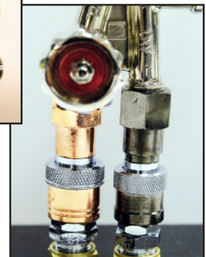
Super Sentinel and Safety-Z Coupling Sets
